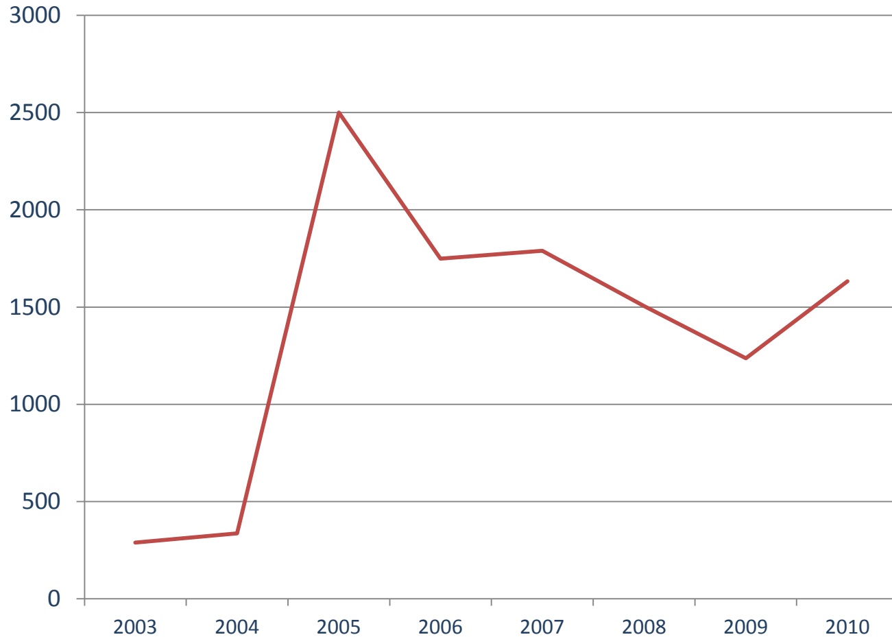
Submissions/year
