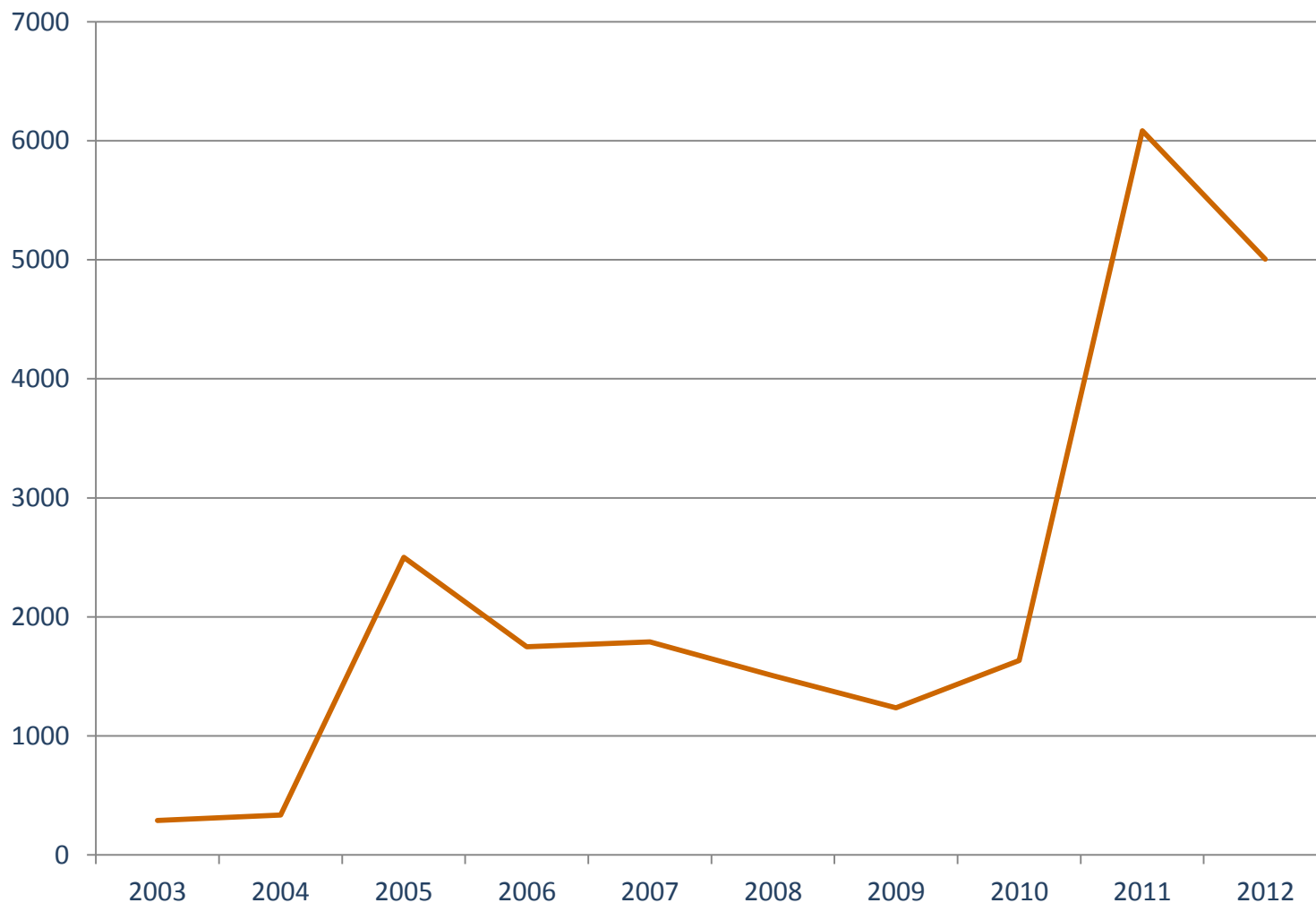
Submissions / year
