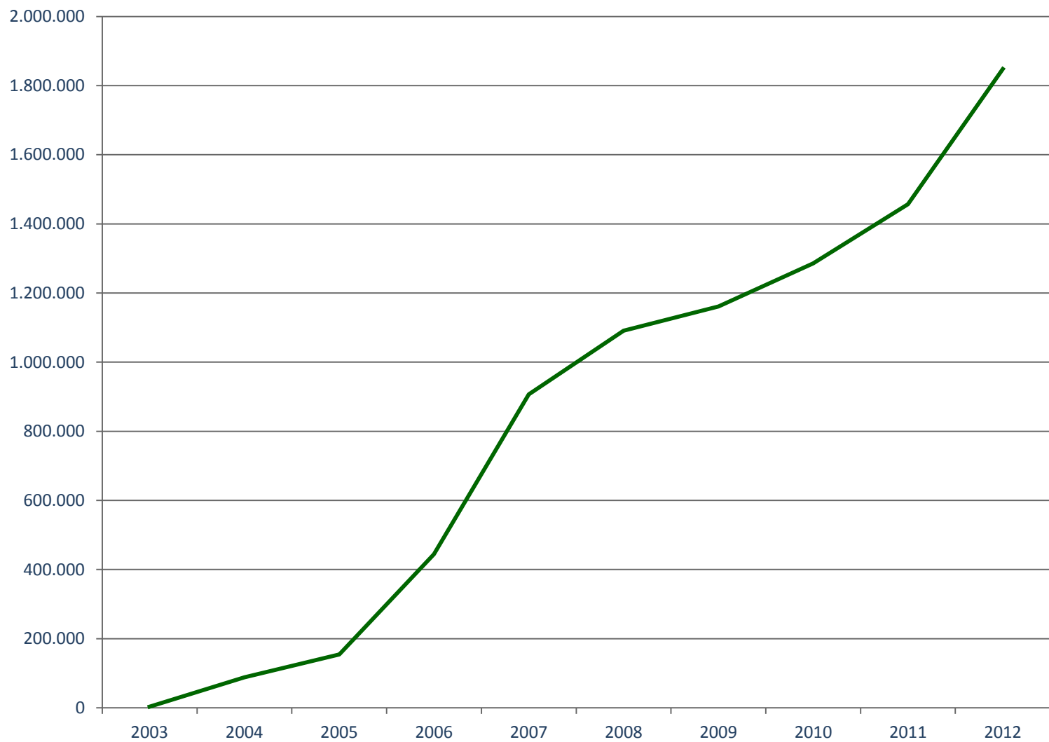
Downloads / year
